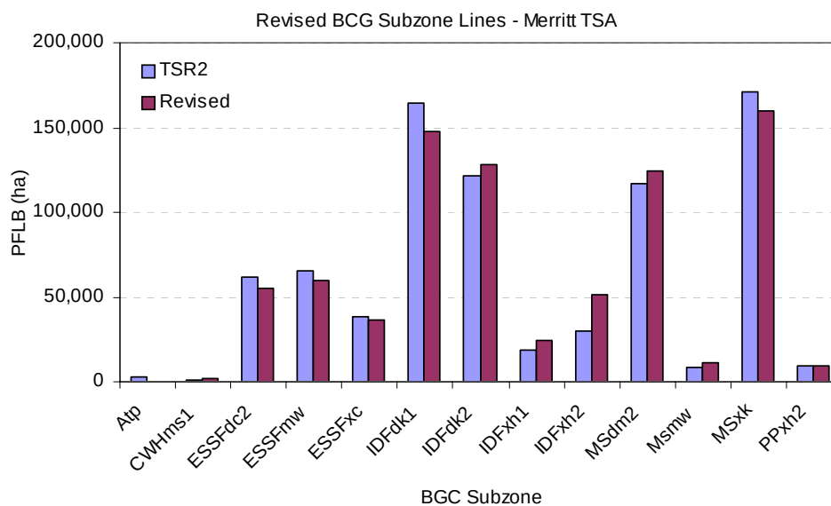
Figure 6. Biogeoclimatic profile (IFPA AAC application).
