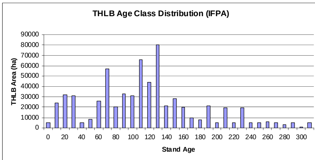
Figure 4. Age class distribution (TSR2 – 2001).
